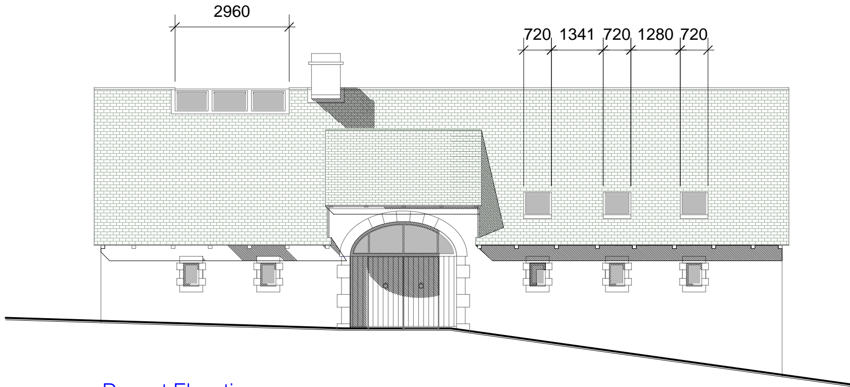
Devant Elevation
